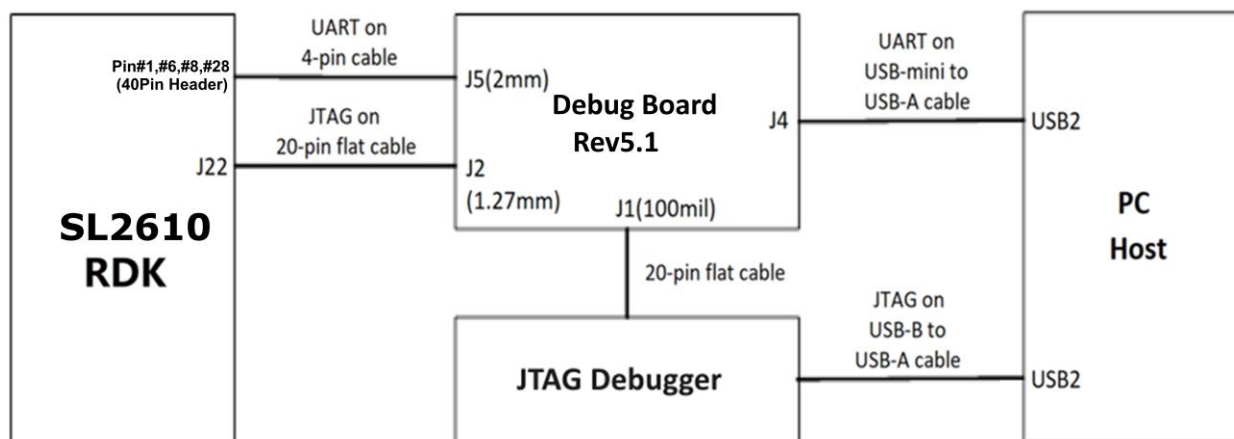
Figure 14. Debug board connectivity for UART and JTAG
