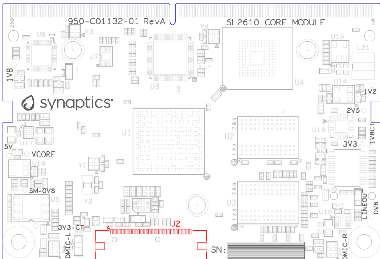
Figure 10. Locations on core module top side
