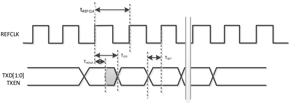
Figure 16. RMII timing
