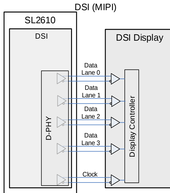
Figure 29. DSI connectivity
