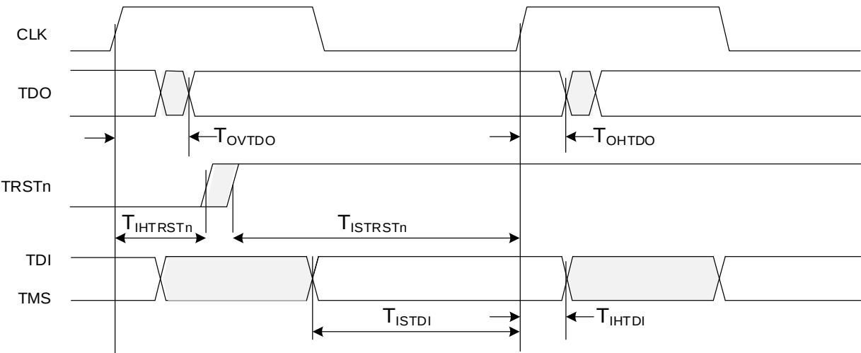
Figure 17. JTAG timing
