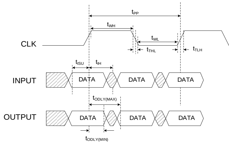
Figure 23. eMMC Timing – High-speed dual-rate interface
