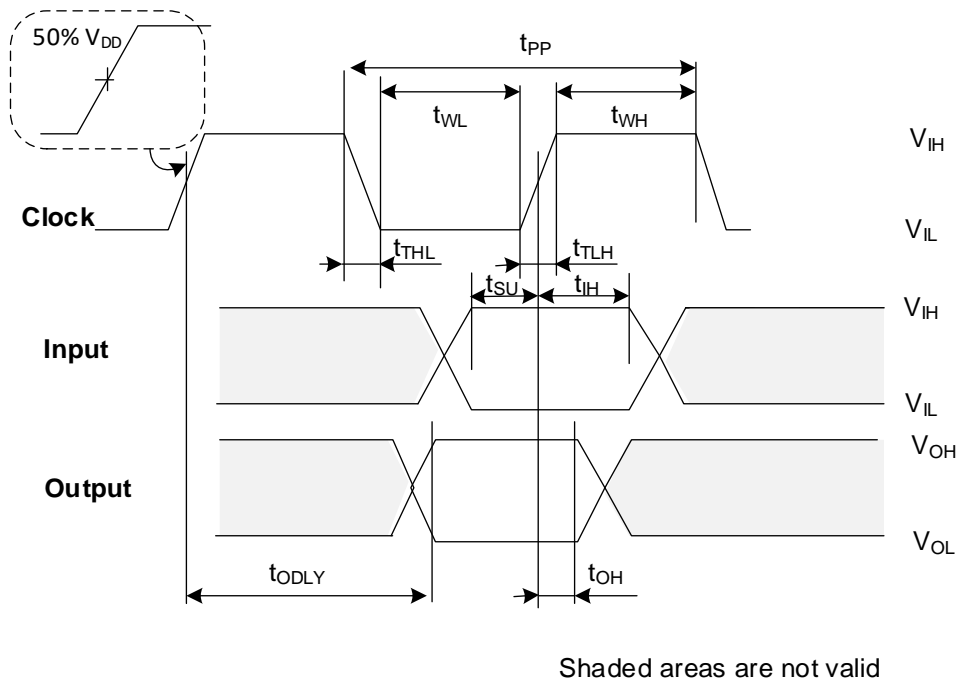
Figure 11. Timing Diagram Data Input/Output Referenced to Clock (High-speed)
