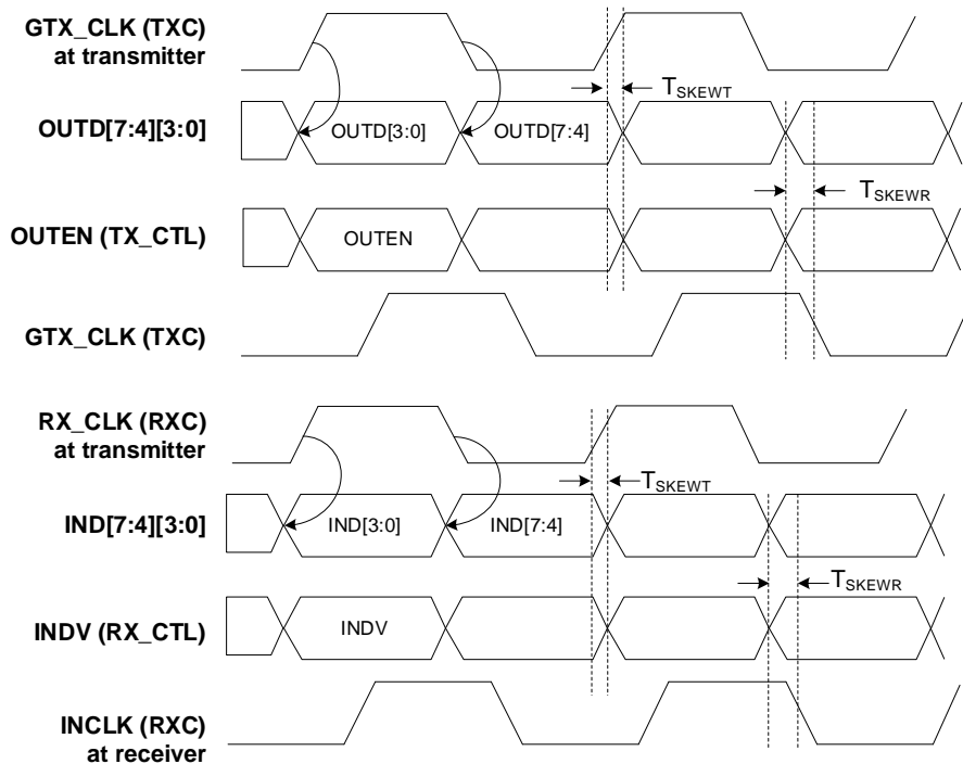
Figure 16. RGMII Timing
