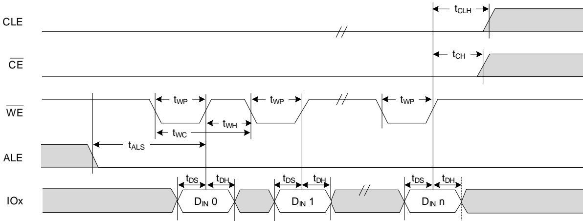
Figure 25. Data Input Cycle Timing
