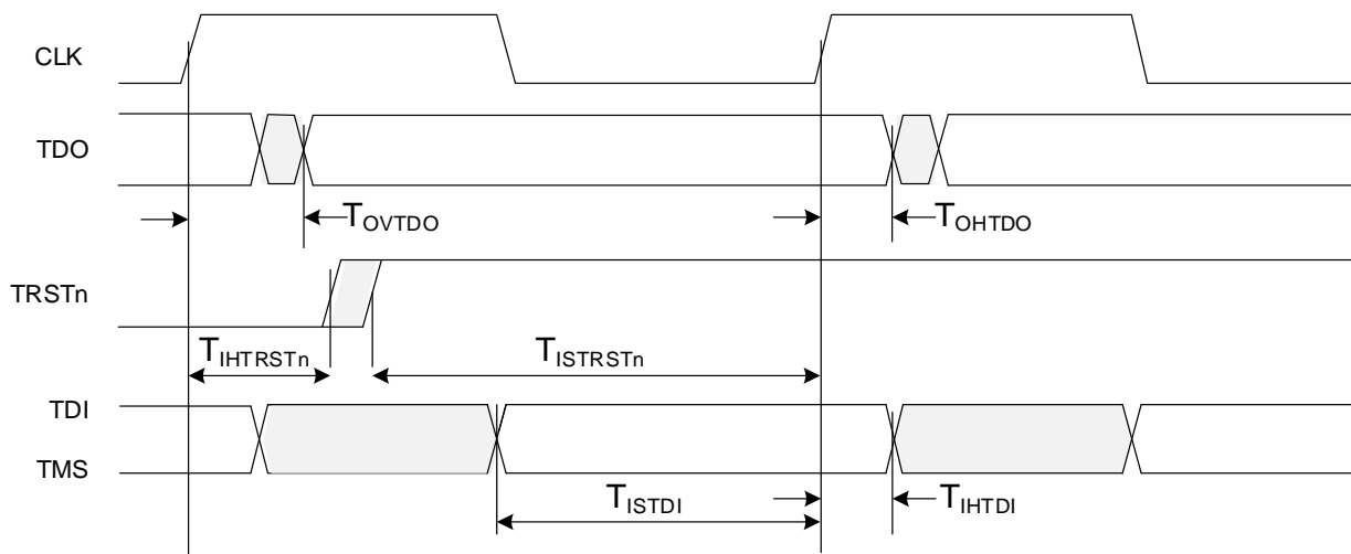
Figure 17. JTAG Timing
