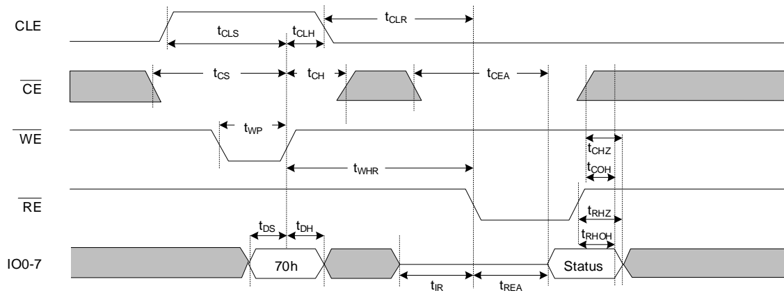
Figure 28. Read Status Timing
