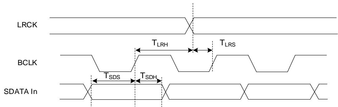
Figure 19. I 2 S slave mode timing
