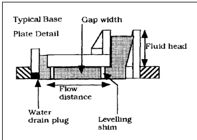
DRAWING 1.1
