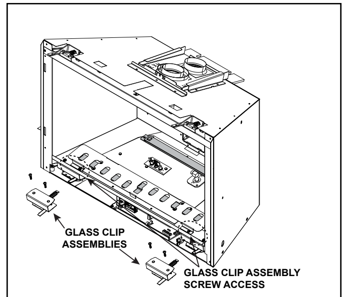
Figure 4.5 Glass Clip Assembly Removal
