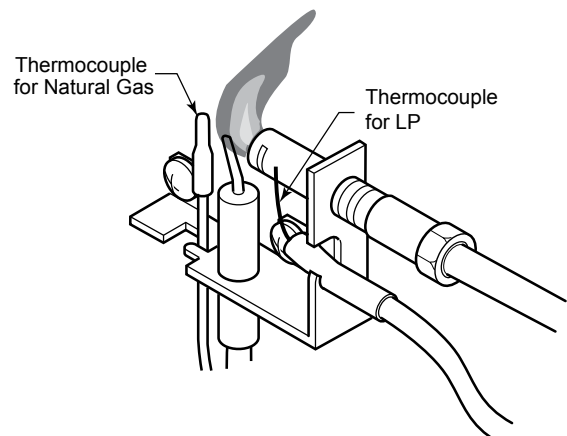
Figure 11.2 Incorrect Pilot Flame Appearance
