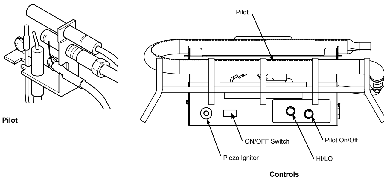
Figure 10.2 - Piezo Ignitor
