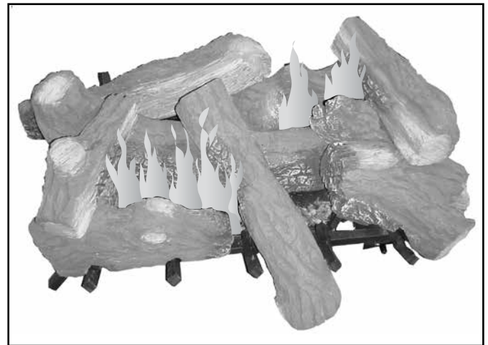
Figure 5.12 - Correct Appearance of Rear Flames
