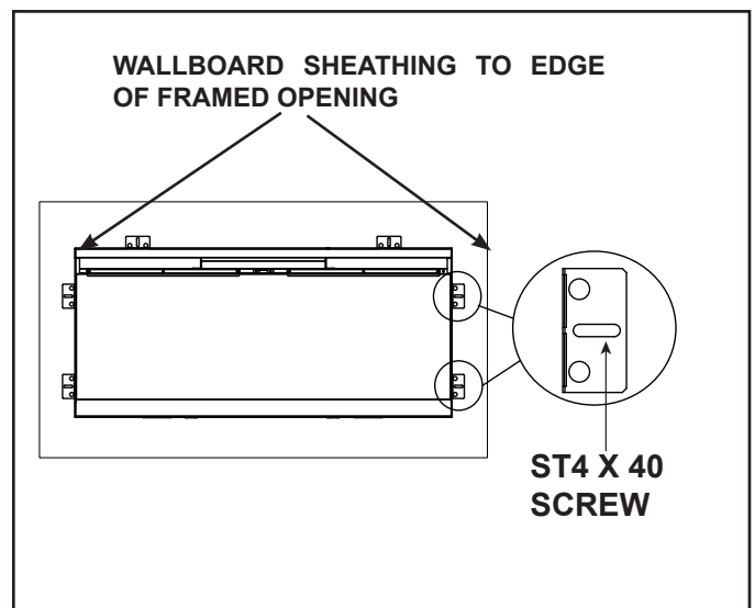
Figure 4.3 Fasten Appliance to Framing
