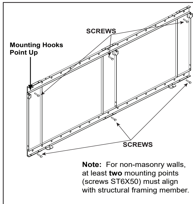
Figure 4.8 Bracket Attachment
