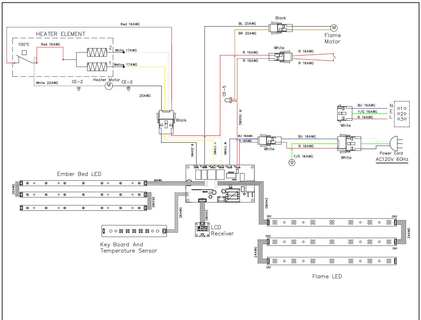
Figure 6.1 Wiring Diagram
