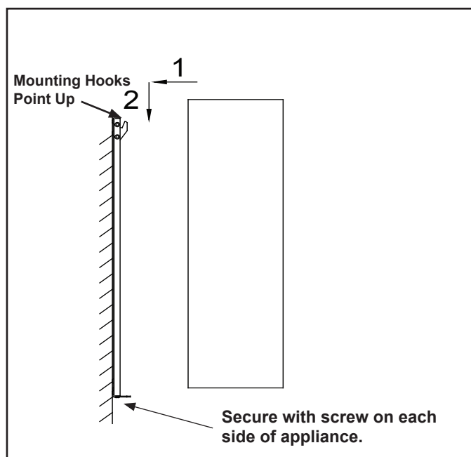
Figure 4.9 Attaching Appliance to Bracket
