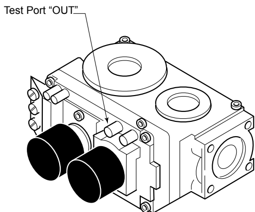
Figure 4.2 - Pressure Test Point Location Millivolt Control
