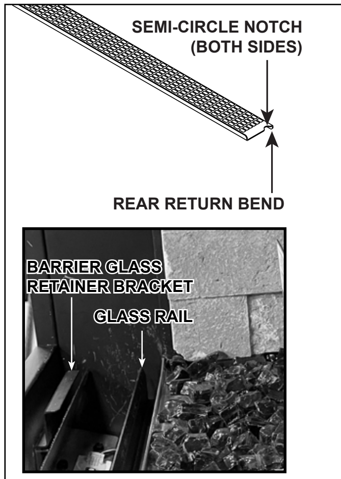
Figure 11.19 Install Transition Media Tray
