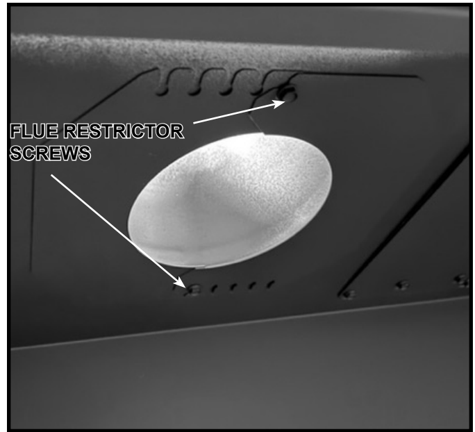
Figure 4.15 Flue Restrictor Installed
