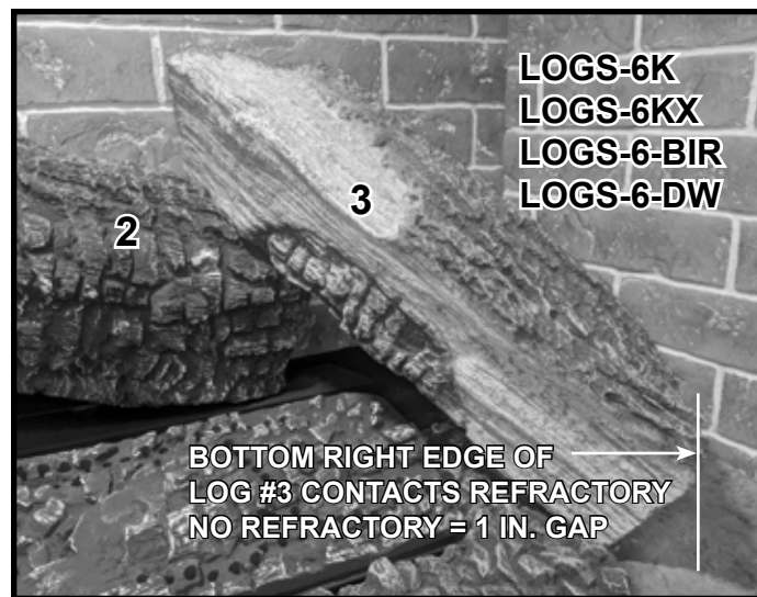
Figure 5.B Place Log #3 (LOGS-6K / LOGS-6KX / LOGS-6-BIR / LOGS-6-DW)
