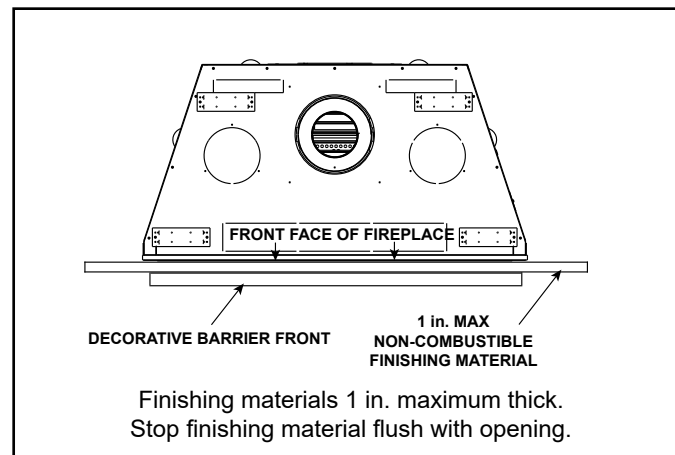
Figure 10.13 Overlap Fit Decorative Barrier Front
