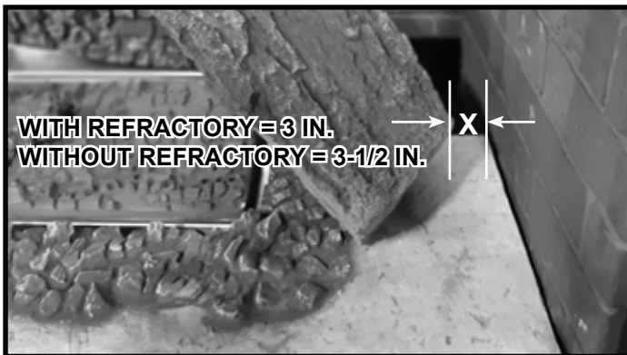
Figure 6 Place Log #3 (LOGS-8K / LOGS-8KX / LOGS-8-BIR / LOGS-8-DW)
