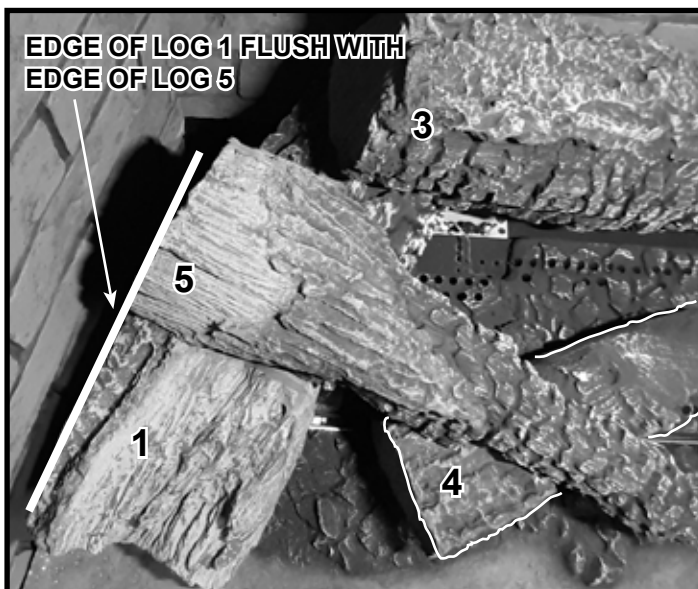
Figure 10 Place Log #5 (LOGS-6K / LOGS-6KX / LOGS-6-BIR / LOGS-6-DW)
