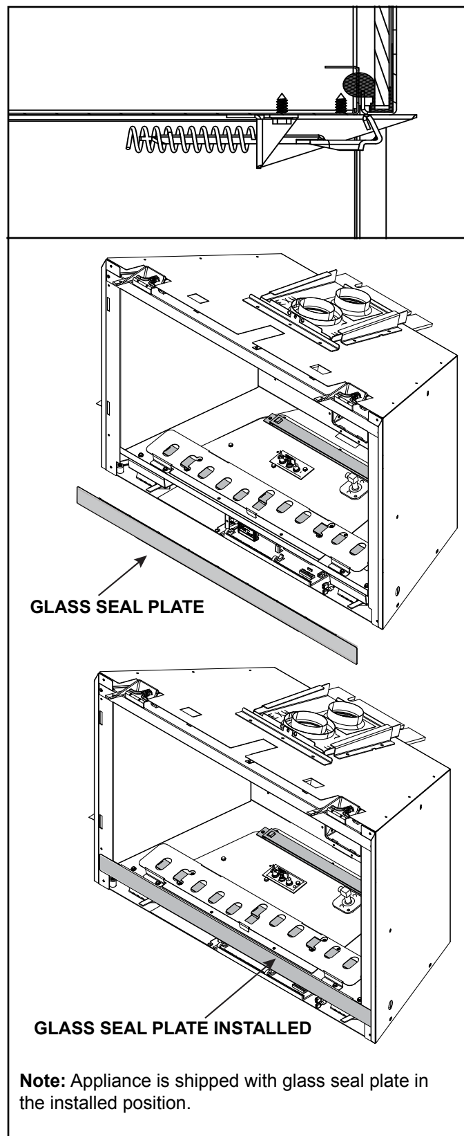
Figure 9.2 Glass Seal Plate
