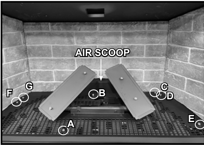
Figure 2 Log Pin Locations
