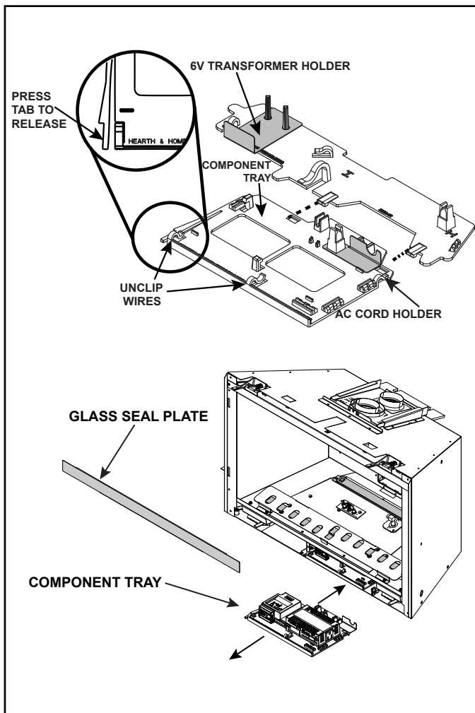
Figure 7.3 Component Tray
