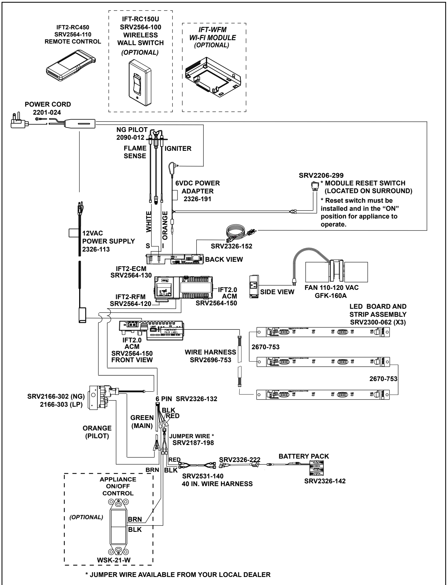
Figure 6.2 IntelliFire Touch 2.0 Wiring Diagram - SUPREMEX-I30
