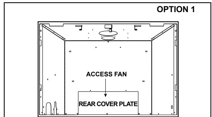
Figure 6.3 Cover Plate Removed (Option 1)
