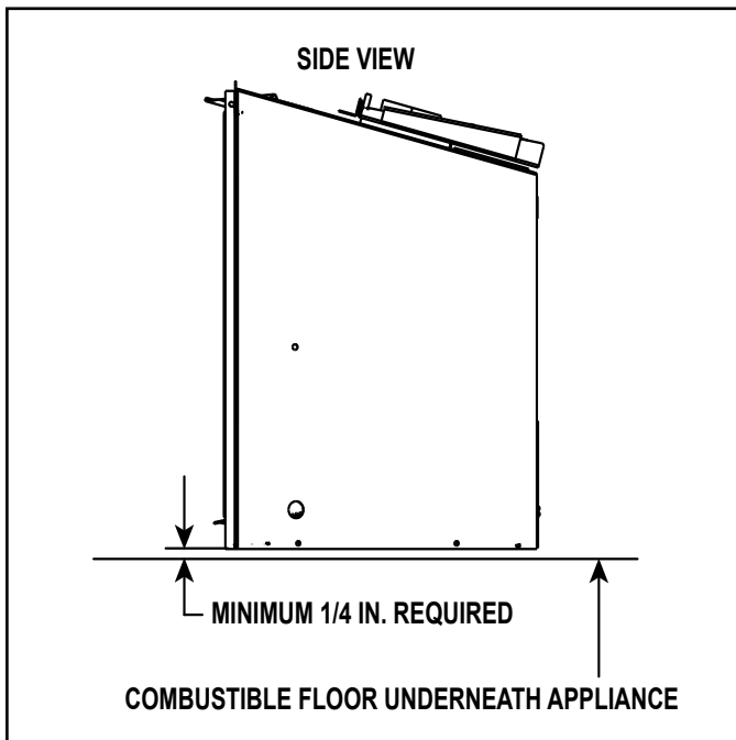
Figure 3.19 Solid Fuel Combustible Floor Clearance
