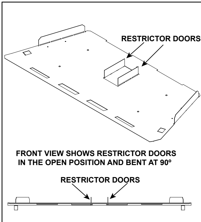
Figure 9.3 Firebox Baffle with Restrictor Doors Open
