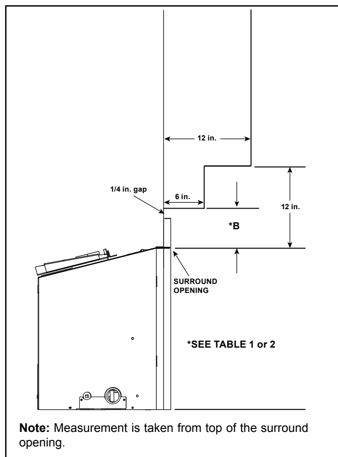
Figure 8.2 Minimum Vertical and Maximum Horizontal Dimensions- Non-Combustible
