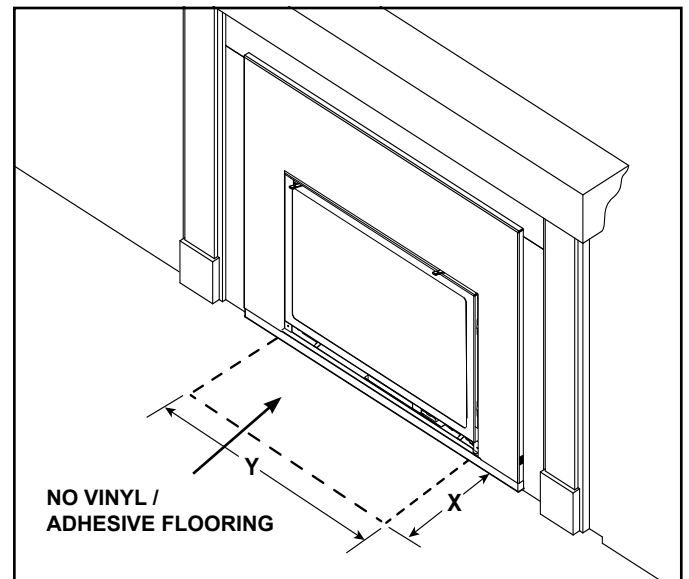
Figure 3.21 Hearth - Combustible Material Exception
