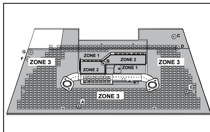
Figure 11 Zone 3 Media Placement
