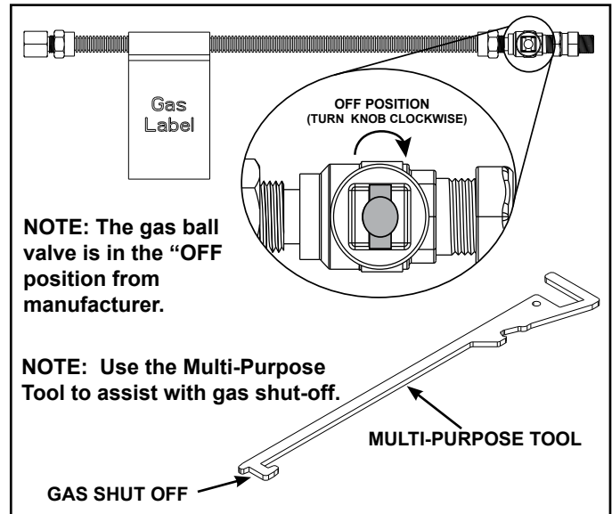
Figure 7.1 Gas Shut-off
