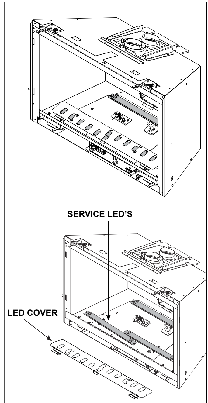
Figure 6.6 Service LED's
