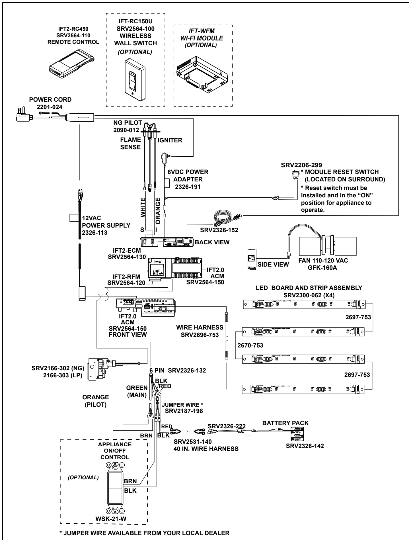
Figure 6.2 IntelliFire Touch 2.0 Wiring Diagram - SUPREMEX-I35
