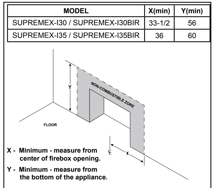
Figure 3.11 Non-Combustible Facing Requirement
