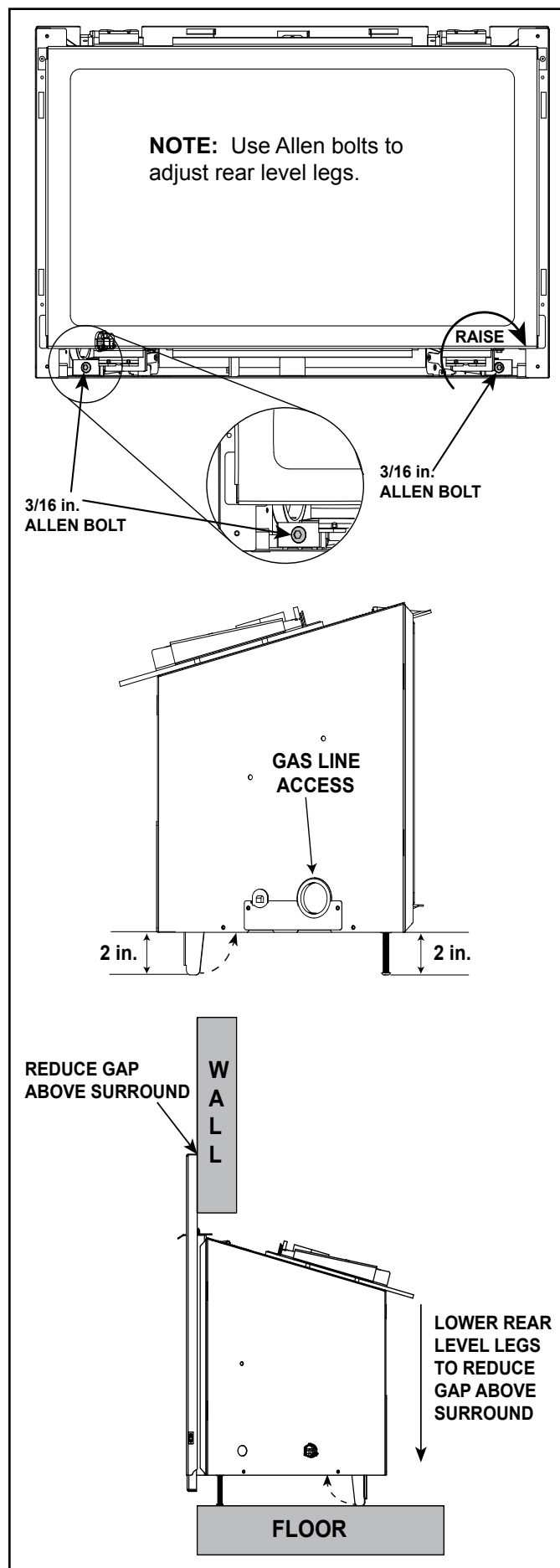
Figure 5.6 Leveling Leg Detail
