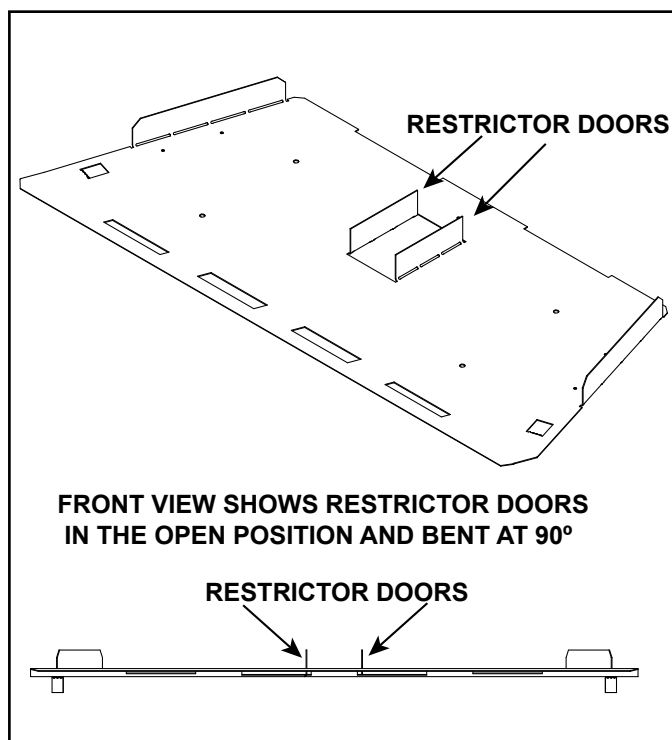
Figure 5.2 Firebox Baffle with Restrictor Doors Open
