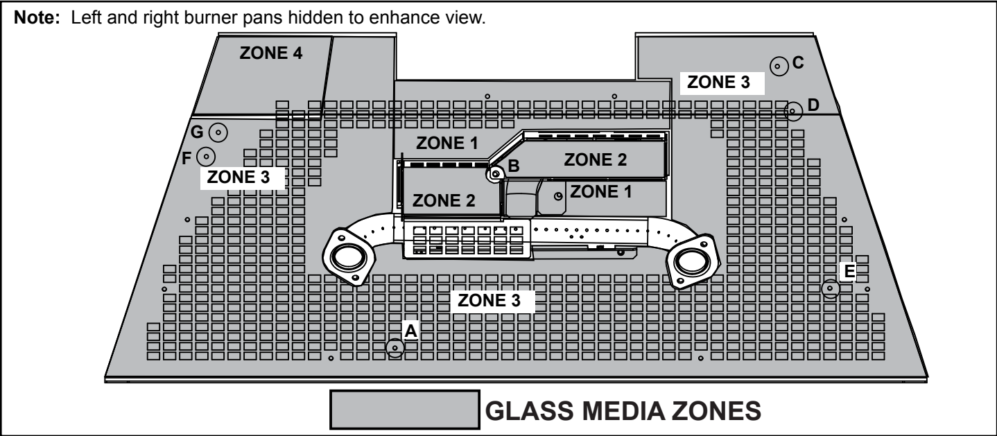
Figure 17 Zone 4 Media Installed
