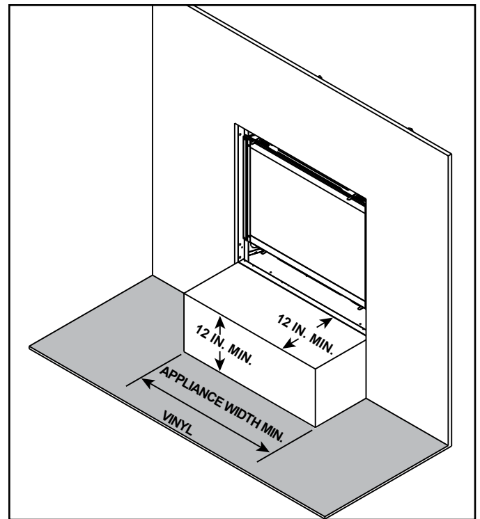
Figure 3.20 Vinyl Flooring Recommendations
