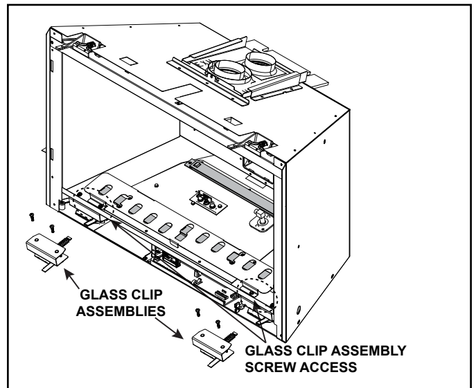
Figure 7.2 Glass Clip Assembly Removal
