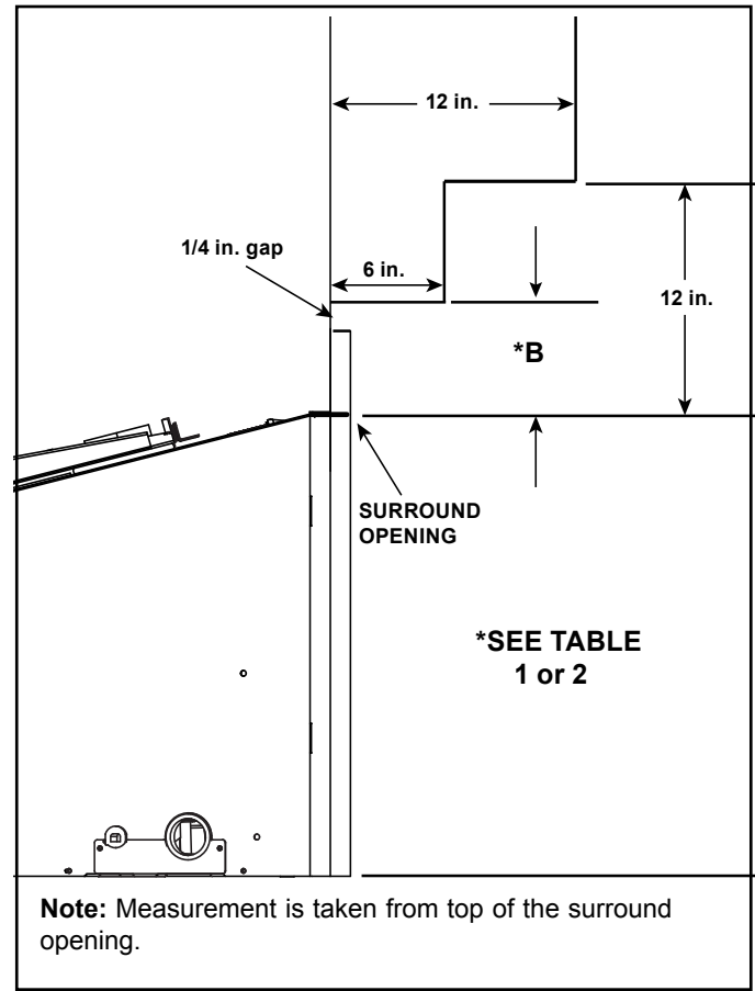
Figure 3.15 Minimum Vertical and Maximum Horizontal Dimensions - Non-Combustible
