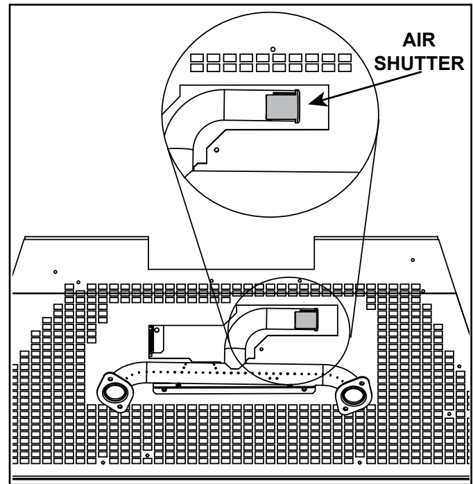
Figure 7.5 Air Shutter
