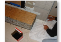
Building a new hearth out of plywood, followed by wire mesh, anchoring to floor, scratchcoat, then stone.
