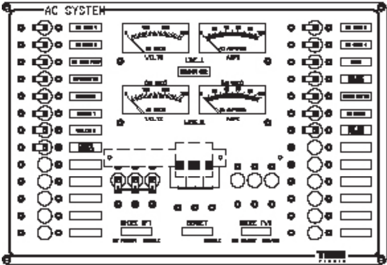
Figure 4-3: A.C. System Panel.
