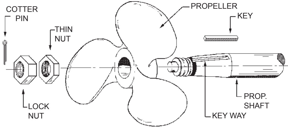
Figure 6-2: Propeller Instalation
