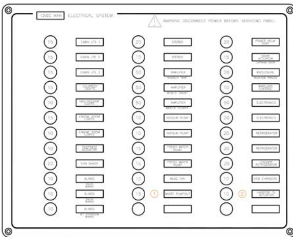
DC distribution panel
