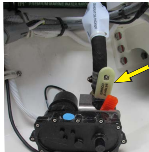
Generator seacock valve with manual override lever
