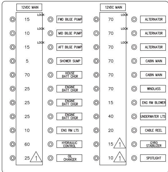
Typical Master DC Panel schematic, Yamaha engine package (see also Appendix F)
