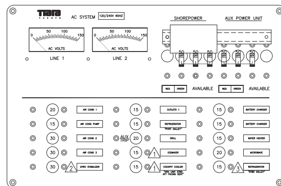
Typical AC distribution panel schematic (see also Appendix F)
