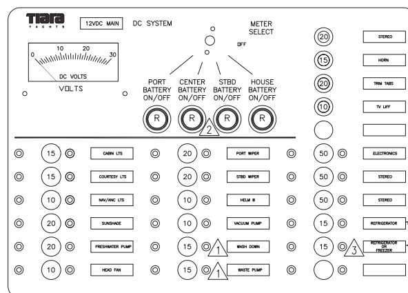
Typical DC distribution panel schematic (see also Appendix F)
