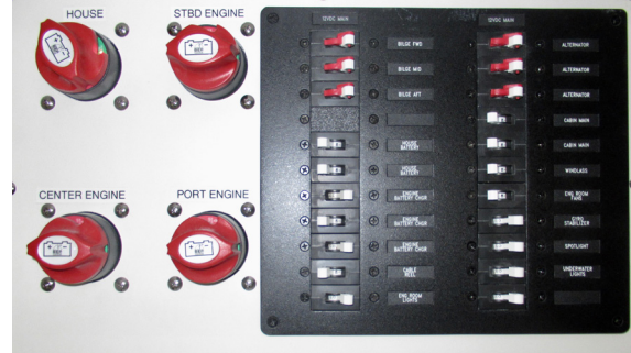
Master DC Panel
