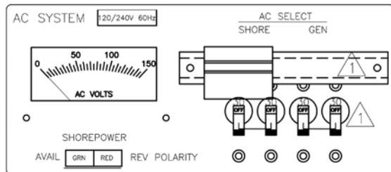
Shore power and generator select switch and polarity indicator lights
