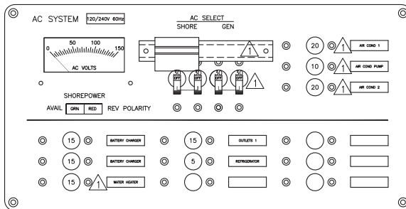
AC distribution panel
