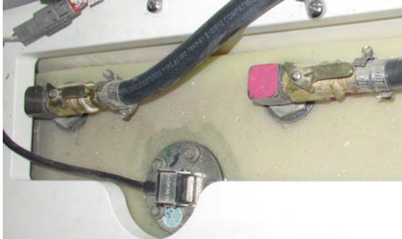
Generator fuel supply and return valves
