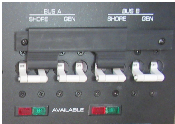
Shore power and generator indicator lights, on the AC distribution panel (typical)
