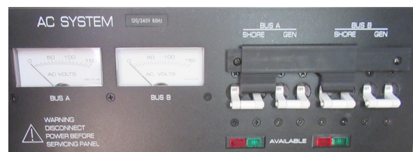
Shore power and generator select switches and polarity indicator lights
