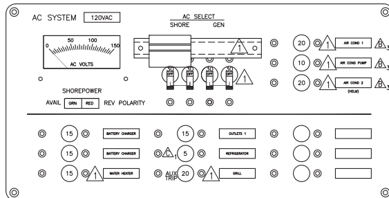
AC distribution panel schematic
