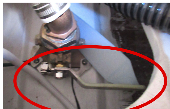
Waste discharge seacock
