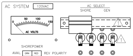
Detail of AC distribution panel schematic: shore power and generator power AC select switch and polarity indicator lights
