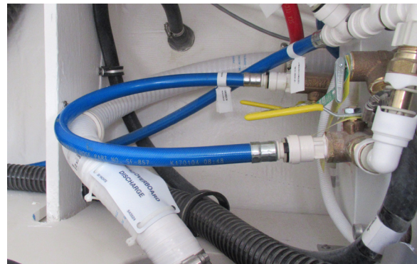
If installed, the optional waste discharge seacock is located aft of the water heater
