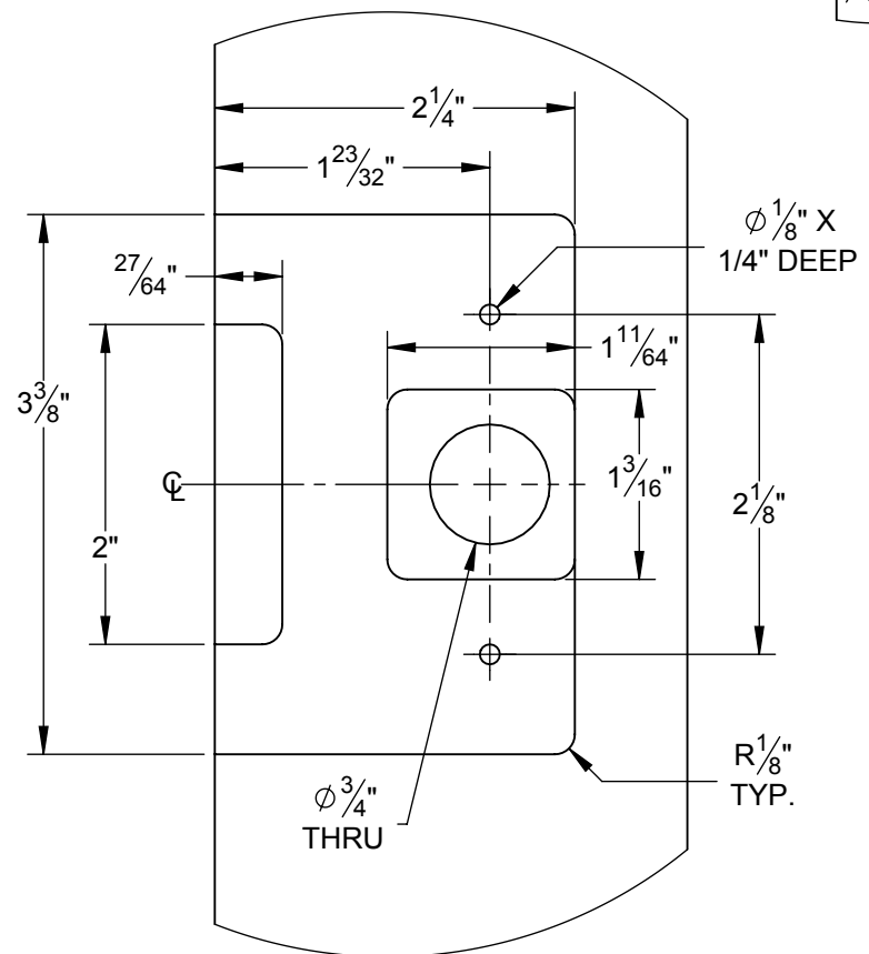
DETAIL B SCALE 3 : 4
