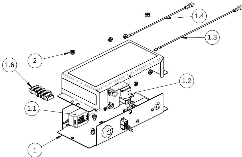
DOUBLE SIDE BURNER ELECTRICAL BOX SHOWN FOR REFERENCE
