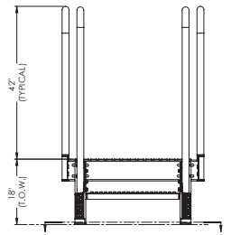
Front Elevation View
