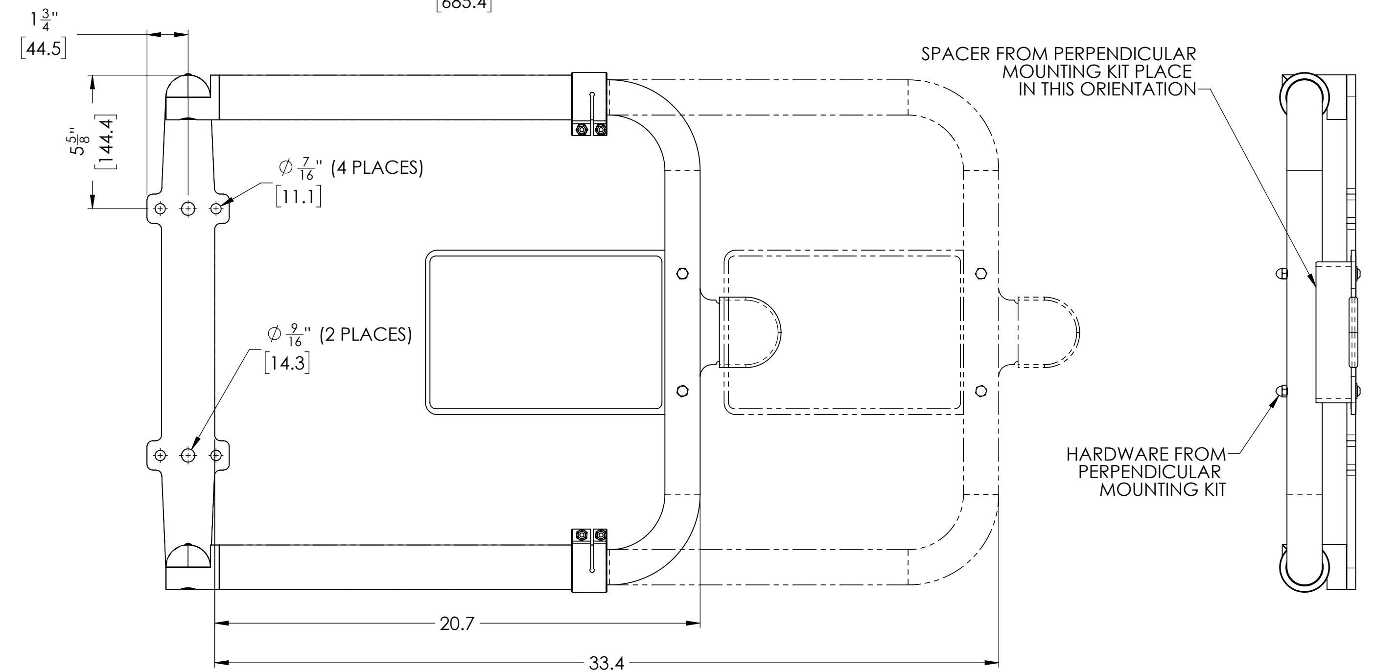
PERPENDICULAR MOUNTING CONFIGURATION CUSTOMER / FIELD OPTIONAL CONFIGURATION
