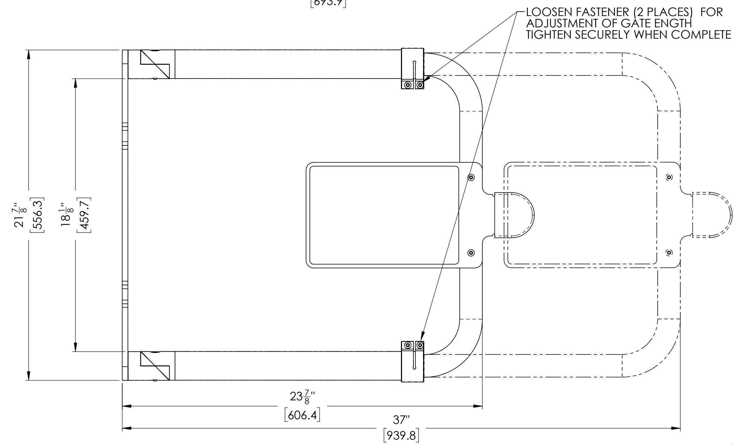
PARALLEL MOUNTING CONFIGURATION FACTORY SETTING / CONFIGURATION
