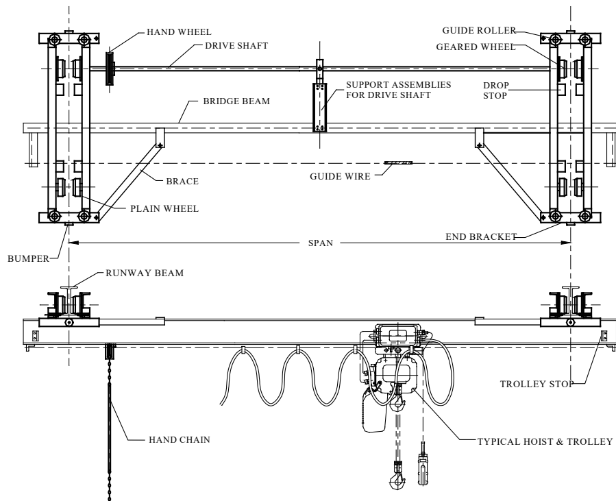
TYPICAL CRANE SYSTEM WITH UNDERHUNG GEARED END TRUCKS
