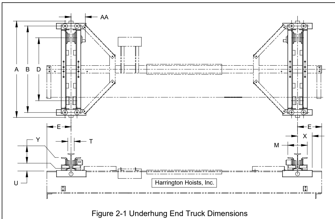
Underhung Push (Manual) End Trucks (Refer to Fig. 2-1)
