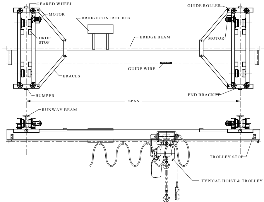
TYPICAL CRANE SYSTEM WITH UNDERHUNG MOTORIZED END TRUCKS
