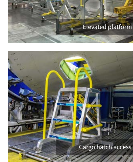
Starliner assembly
