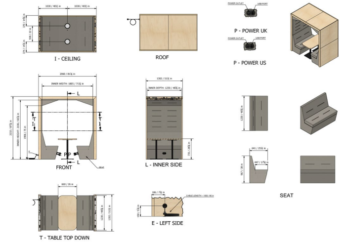
4 Person, Arch Roof, Open Back, with Spotlights
