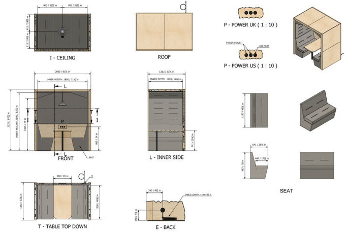
4 Person, Arch Roof, Upholstered Back, with Pendant
