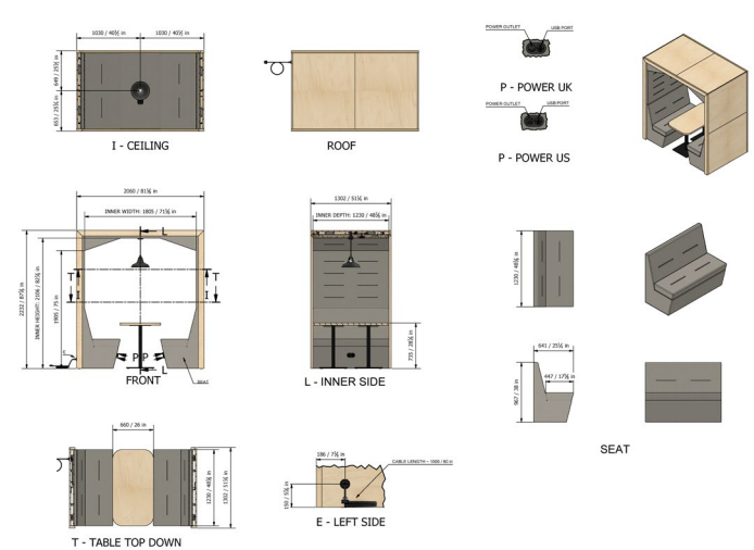
4 Person, Arch Roof, Open Back, with Pendant
