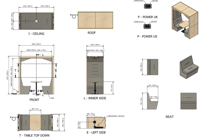
2 Person, Arch Roof, Open Back, with Spotlight
