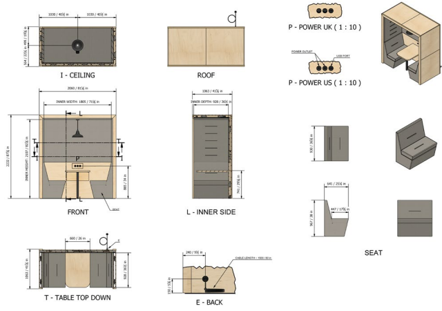
2 Person, Flat Roof, Upholstered Back, with Pendant
