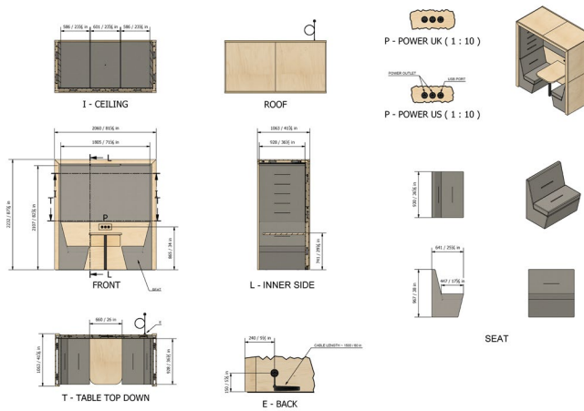
2 Person, Flat Roof, Upholstered Back, with Striplight
