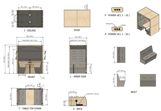
4 Person, Arch Roof, Upholstered Back, with Spotlights
