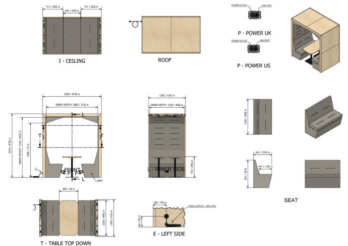
4 Person, Arch Roof, Open Back, with Striplight
