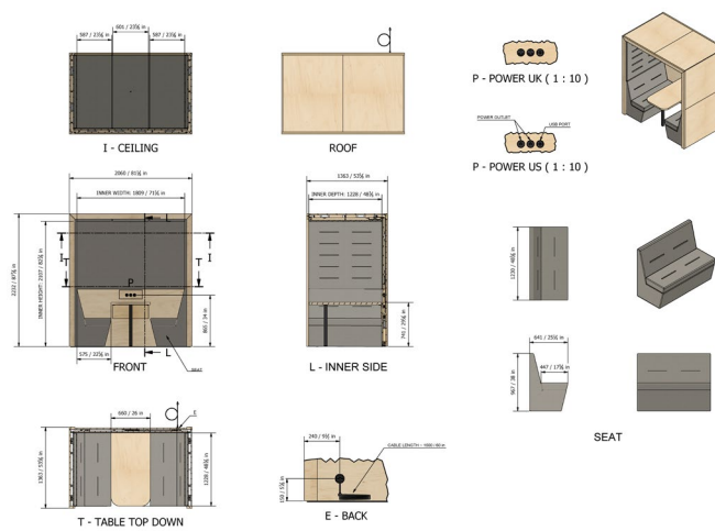
4 Person, Flat Roof, Upholstered Back, with Striplight
