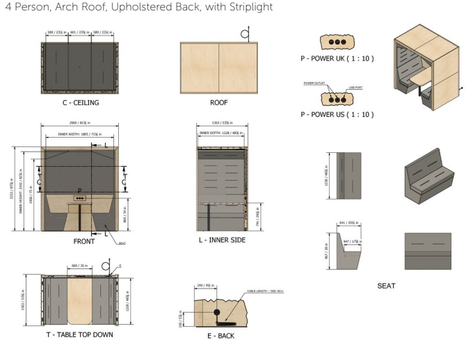
4 Person, Arch Roof, Upholstered Back, with Striplight
