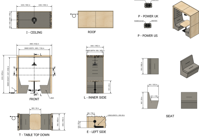
2 Person, Flat Roof, Open Back, with Pendant
