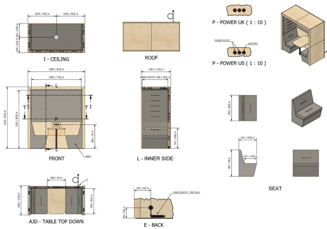
2 Person, Flat Roof, Upholstered Back, with Spotlight
