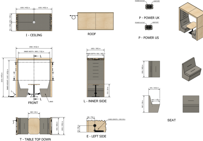
2 Person, Flat Roof, Open Back, with Spotlight
