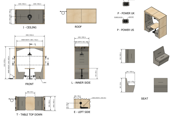
2 Person, Arch Roof, Open Back, with Pendant
