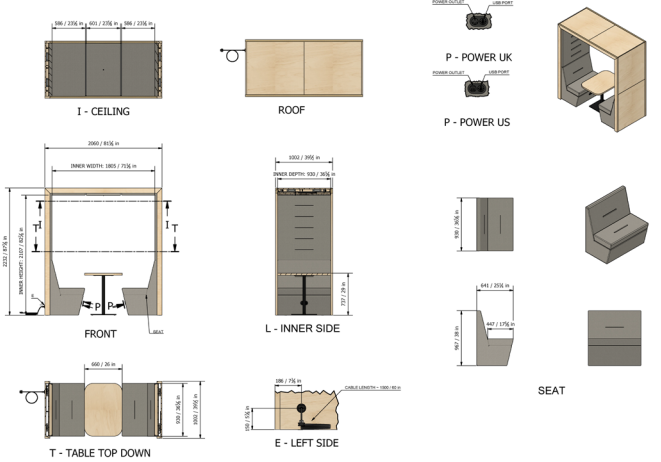
2 Person, Flat Roof, Open Back, with Striplight
