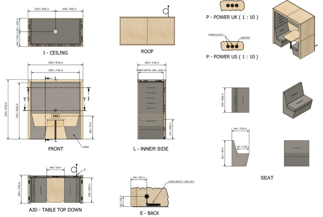
2 Person, Flat Roof, Upholstered Back, with Spotlight
