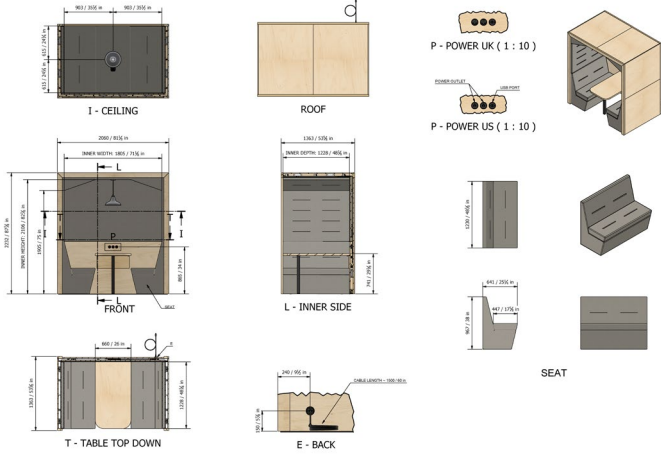
R4 Person, Arch Roof, Upholstered Back, with Pendant
