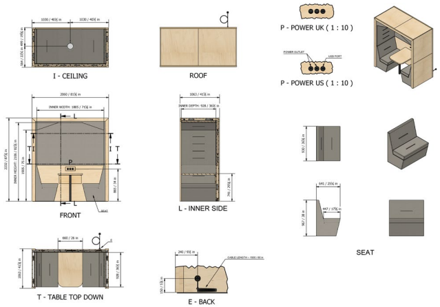
2 Person, Arch Roof, Upholstered Back, with Spotlight
