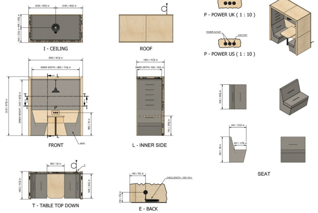
2 Person, Flat Roof, Upholstered Back, with Pendant
