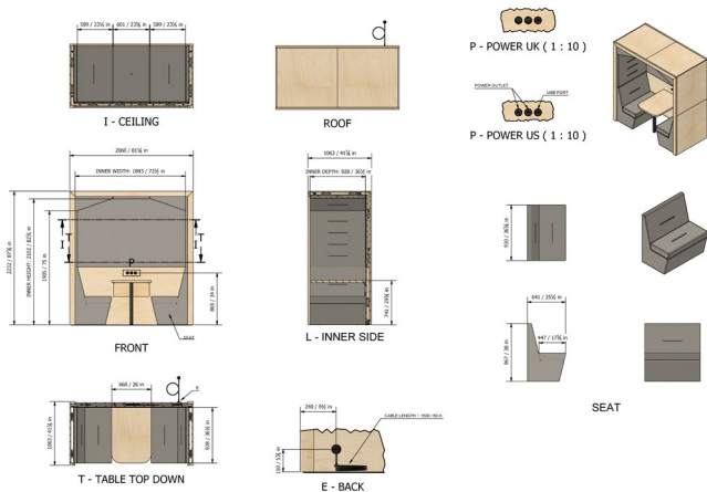
2 Person, Arch Roof, Upholstered Back, with Striplight
