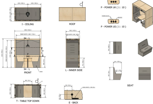
2 Person, Arch Roof, Upholstered Back, with Pendant
