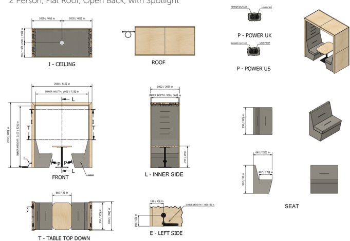
2 Person, Flat Roof, Open Back, with Spotlight
