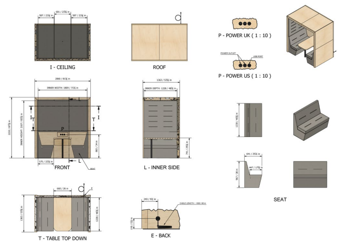
4 Person, Flat Roof, Upholstered Back, with Striplight
