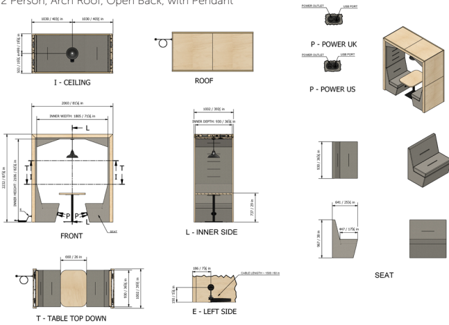
2 Person, Arch Roof, Open Back, with Pendant
