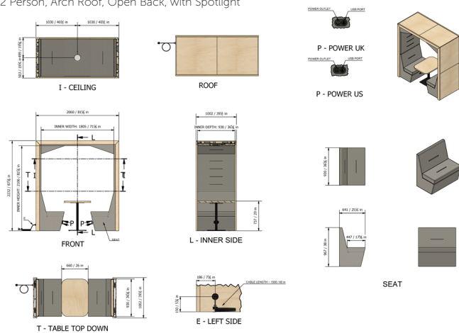
2 Person, Arch Roof, Open Back, with Spotlight
