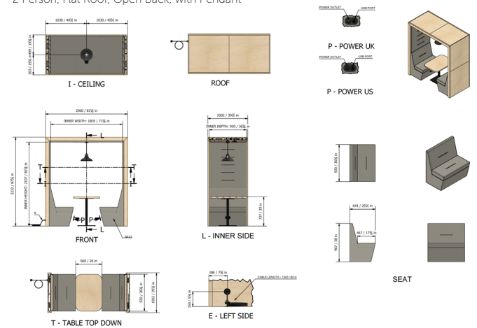
2 Person, Flat Roof, Open Back, with Pendant
