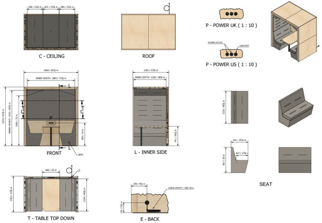
4 Person, Arch Roof, Upholstered Back, with Striplight
