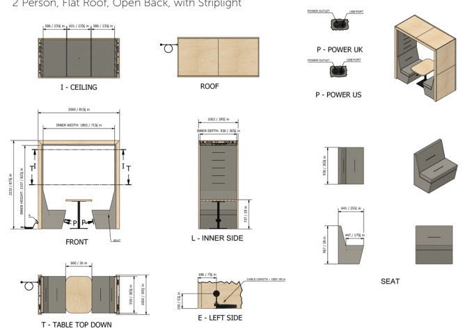
2 Person, Flat Roof, Open Back, with Striplight
