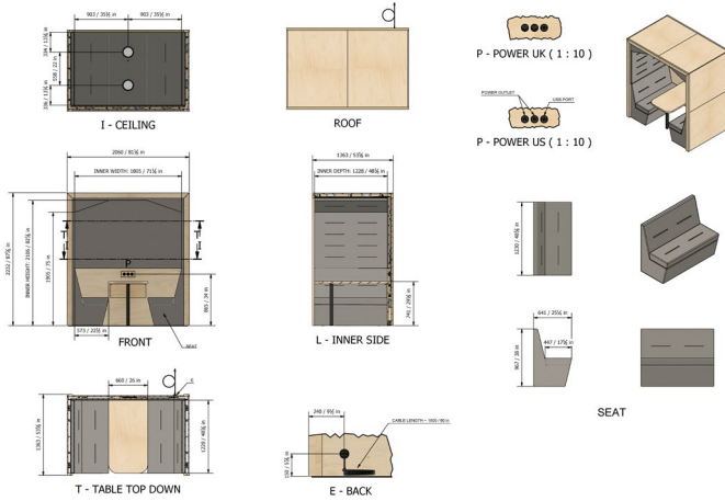
4 Person, Arch Roof, Upholstered Back, with Spotlights
