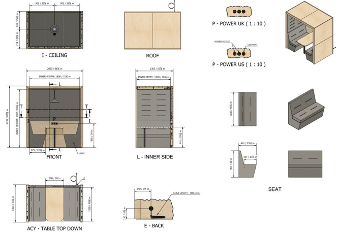
4 Person, Flat Roof, Upholstered Back, with Pendant
