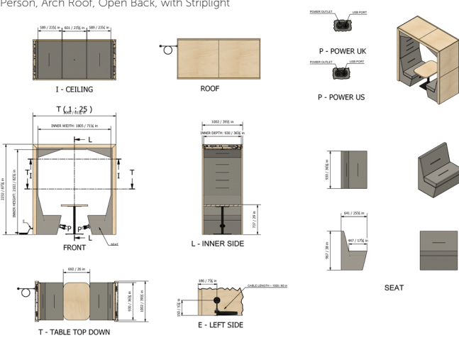
2 Person, Arch Roof, Open Back, with Striplight
