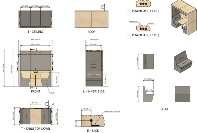
2 Person, Flat Roof, Upholstered Back, with Striplight
