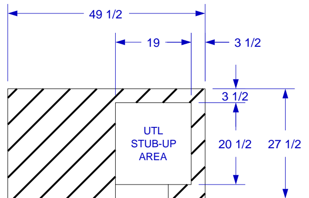
STUB-UP DIAGRAM (SEE NOTE #2)
