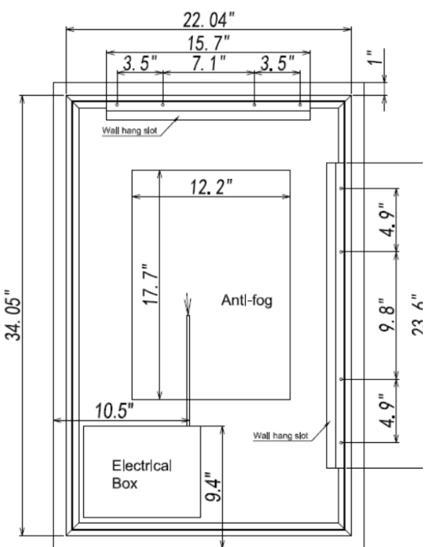
REAR VIEW
