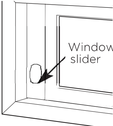
Sliding Window
