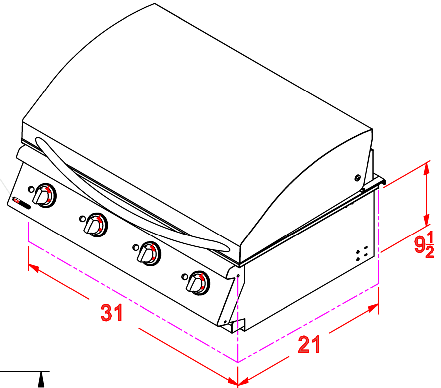
PERSPECTIVE VIEW
