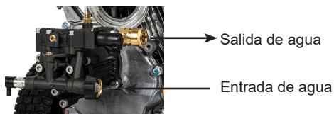
Bomba axial
