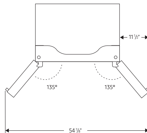
TOP OF REFRIGERATOR WITH DOORS OPEN 135°
