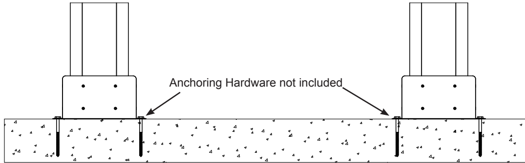
Concrete Patio (min. 11' 6" x 11' 6") with 6" clearance on all sides
