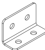
A4M00855 (x1) L BRACKET 32x51x82
