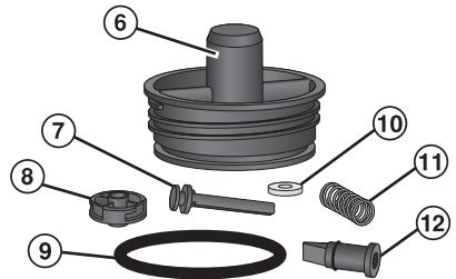
Exploded View of Spirit Bottle Lid Assembly
