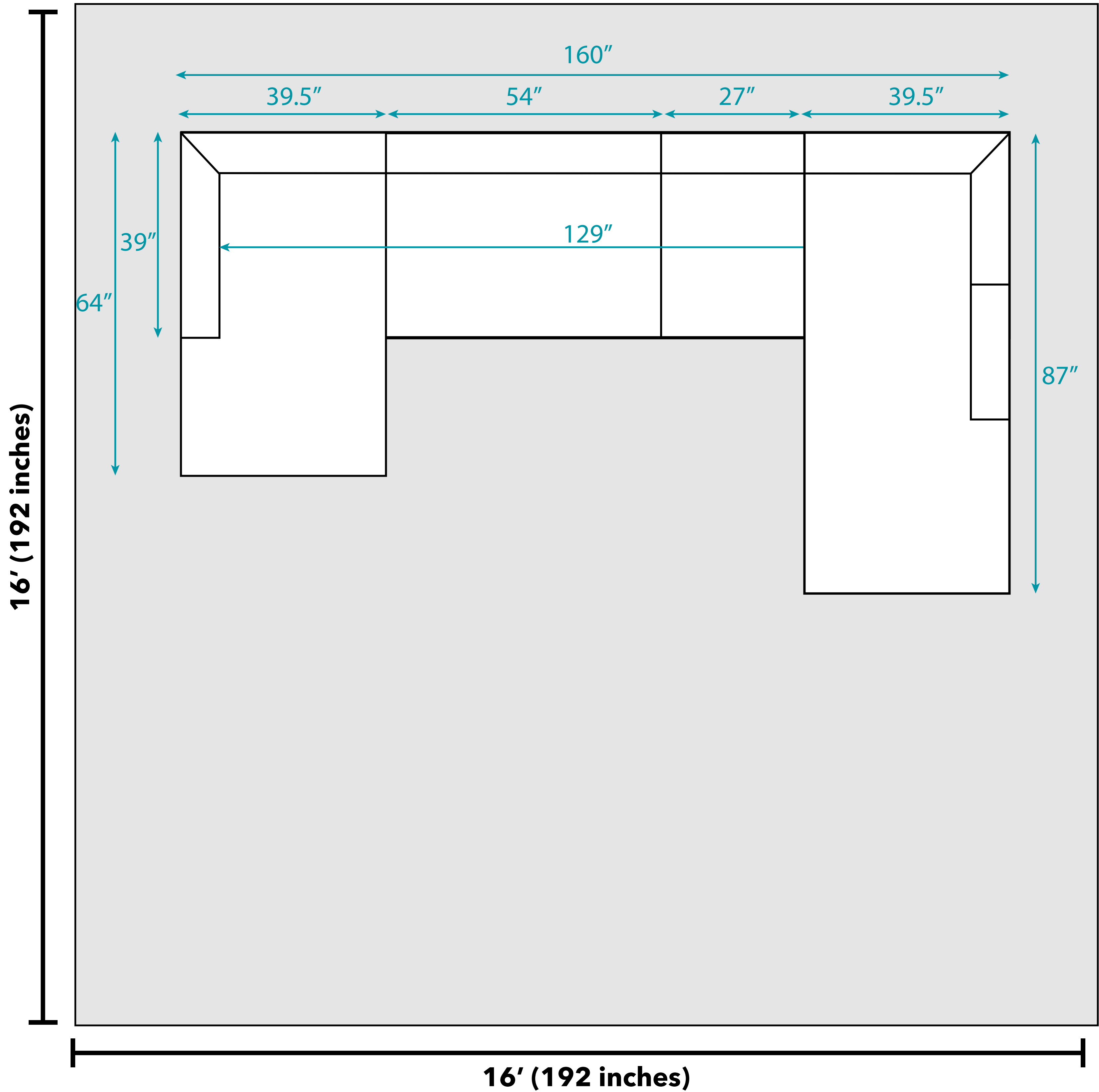
Floor Plan
