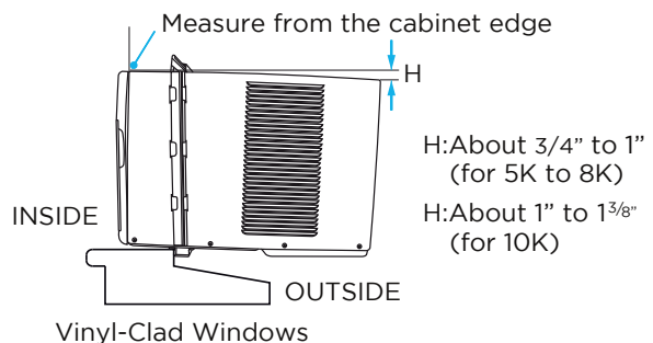
Vinyl-Clad Windows
