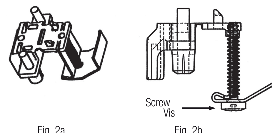
Fig. 2a Fig. 2b Mounting clip. Attache de fixation.
