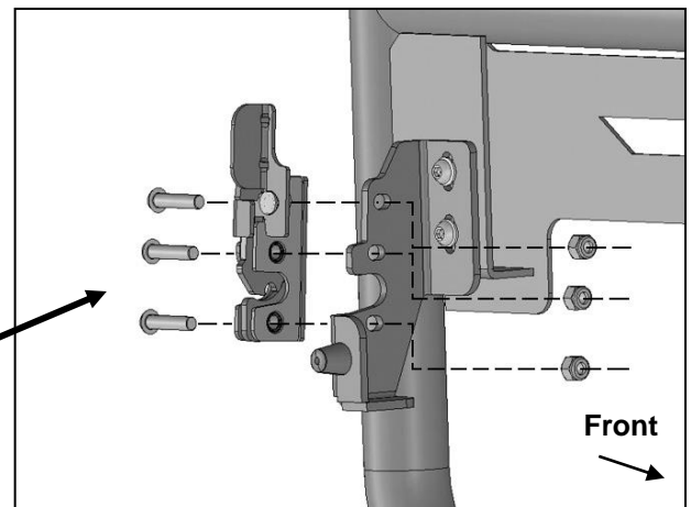
(Fig 9) Attach driver/left Latch to Mounting Bracket
