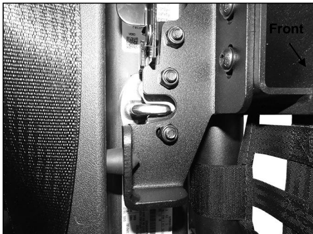
(Fig 14) With Latch fully closed, adjust latch Bracket up or down to rest on striker
