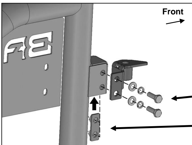
(Fig 5) Attach driver/left Upper Mounting Bracket to mounting tab on back of Door
