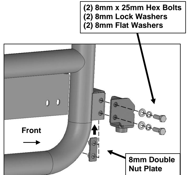
(Fig 7) Attach driver/left Lower Mounting Bracket to mounting tab on back of Door
