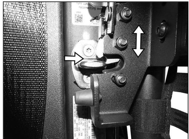
(Fig 13) Open Latch. Adjust latch Bracket up or down for proper operation.
