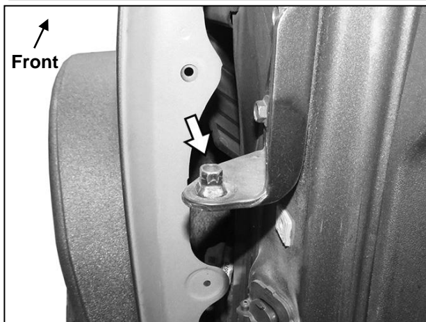
(Fig 3) Driver/left upper door mount
