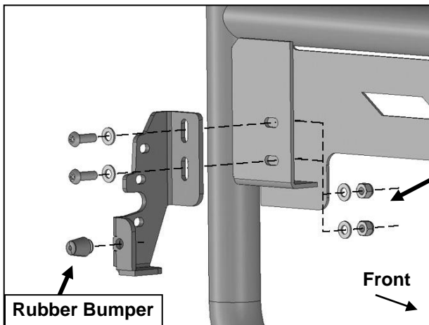
(Fig 8) Attach driver/left Latch Mounting Bracket to mounting tab on back of Door. Push Rubber Bumper into hole in Bracket
