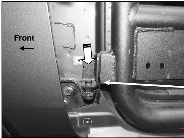
(Fig 12) Attach lower Door Mounting Bracket to door mount (arrow, also see Fig 10)
