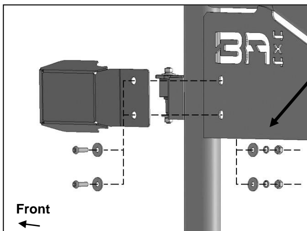
(Fig 15) Attach Upper Hinge Cover to door
