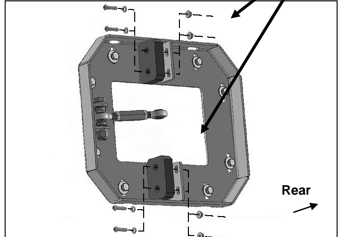
(Fig 9) Attach the Rubber Bump Stops to the Tailgate Mount. Spacers illustrated (arrows) are used for adjustment between the Swing Arm and the Bump Stops only as needed (see Fig 16)
