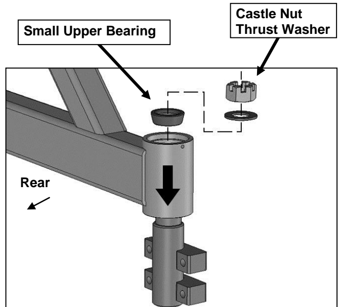
(Fig 16) Slide Swing Arm down over Spindle. Apply grease to Upper Bearing. Insert Upper Bearing into Spindle. Secure Arm to Spindle with (1) Thrust Washer and (1) Castle Nut. Tighten Castle Nut to remove play in Swing Arm
