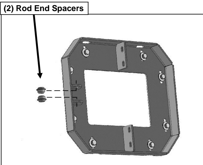
(Fig 7) Insert (2) Rod End Spacers into the holes in the tabs on the Tailgate Mount
