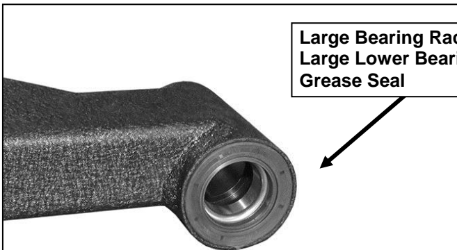
(Fig 15) Insert Bearing Races into Swing Arm. Apply Grease to Lower Bearings. Insert Lower Bearing into Race. Install Grease Seal
