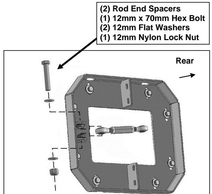
(Fig 8) Slide the end of the Adjuster Assembly between the Rod End Spacers. Attach Adjuster Assembly to tabs and Spacers
