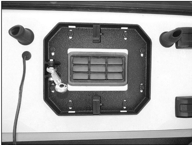
(Fig 10) Tailgate Mount and Adjuster Assembly
