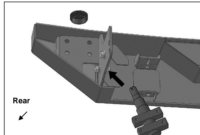
(Fig 11) Remove plug from top of Bumper. Slide Spindle up between mounting plate and back of Bumper. NOTE: It may be necessary to temporarily remove Bumper to install Spindle
