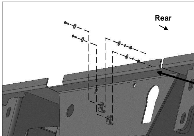
(Fig 10) Attach tire pressure monitoring sensor, if equipped, to tabs on back of bumper
