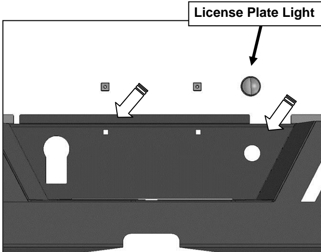
(Fig 13) Push plastic plugs into holes for license plate. Install License Plate Light and trailer plug
