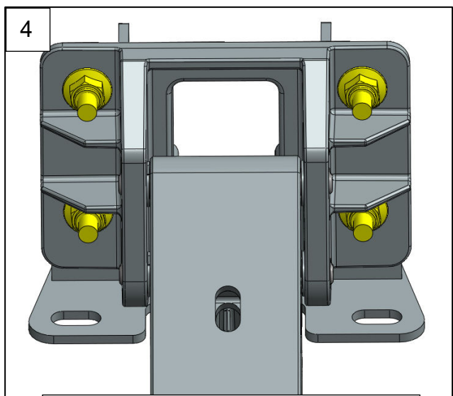
Tighten the M8 Flanged Nylon Lock Nuts all the way until tight.
