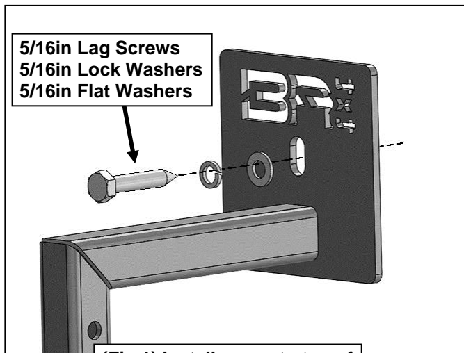
(Fig 1) Install screw to top of Door Storage Bar to wall
