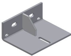
JK Mounting Bracket #1 PN= 4121.02 QTY: 4
