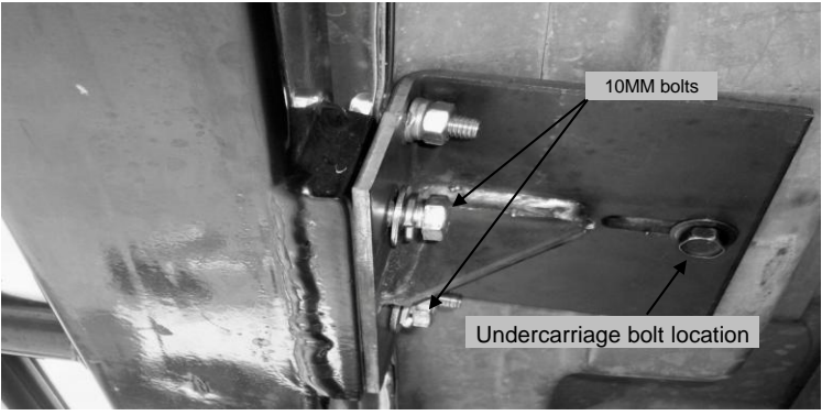
Center Bracket with bar installed
