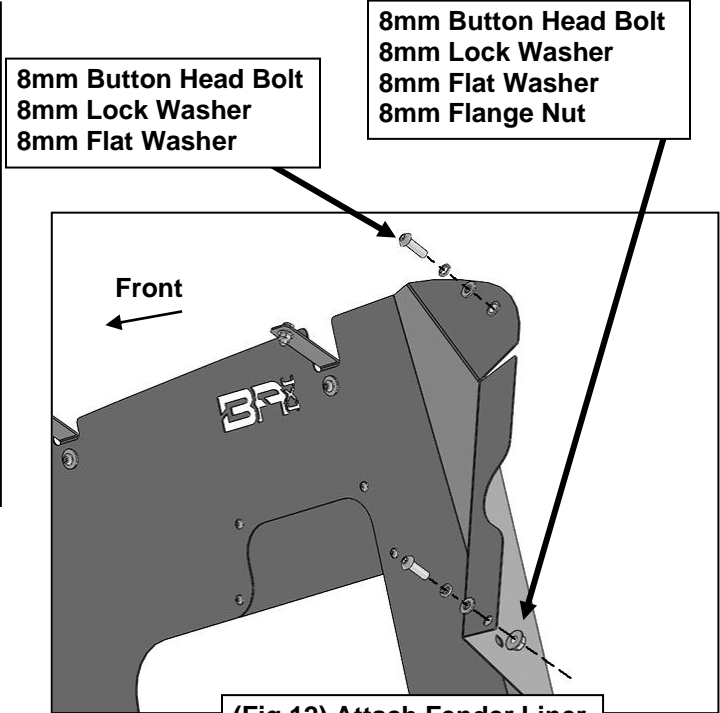
(Fig 12) Attach Fender Liner to back of the wheel well
