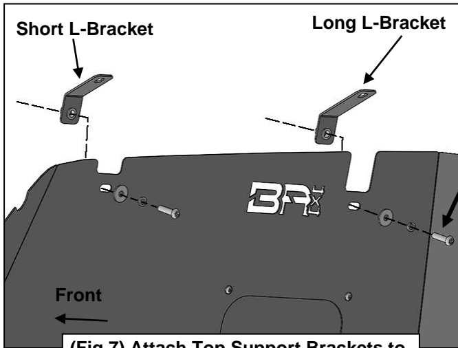
(Fig 7) Attach Top Support Brackets to the top of the Driver/Left Fender Liner
