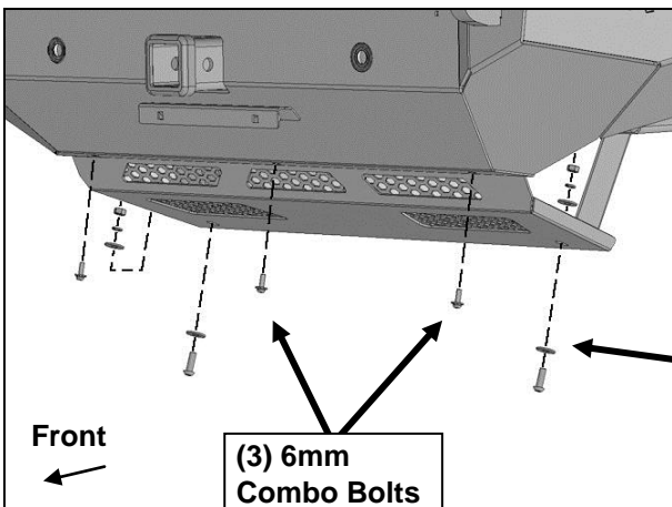
(Fig 21) Attach Skid Plate to back of Bumper and Skid Plate Brackets
