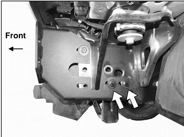
(Fig 5) NOTE: Use Thick Spacer Washers on outer Mounting Bracket (arrows)
