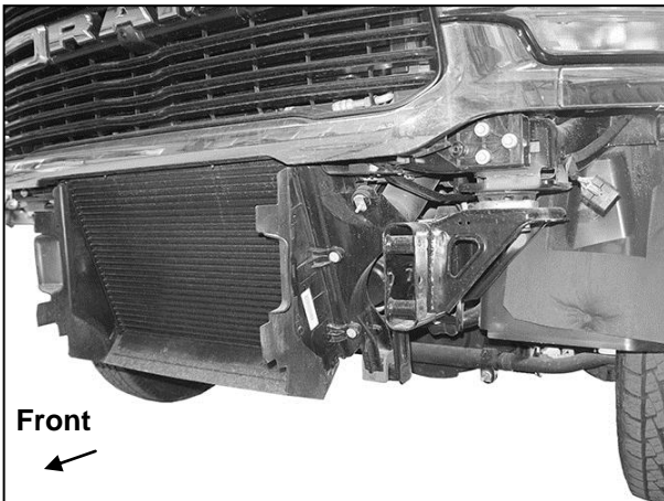
(Fig 3) Bumper assembly removed
