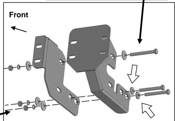
(Fig 4) Attach driver/left Outer and Inner Frame Mounting Brackets to sides of frame. NOTE: Use Thick Spacer Washers on outer Mounting Bracket (arrows)
