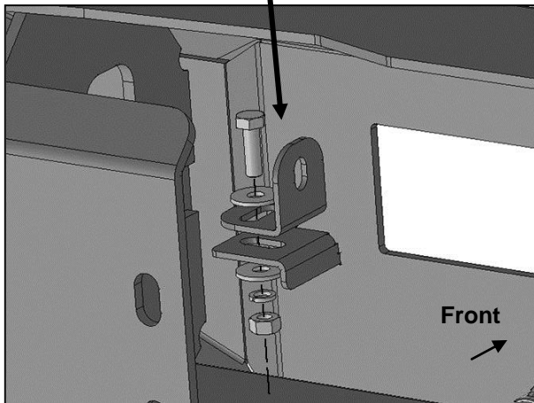
(Fig 11) Attach "L" Bracket to mounting tabs on back of Bumper
