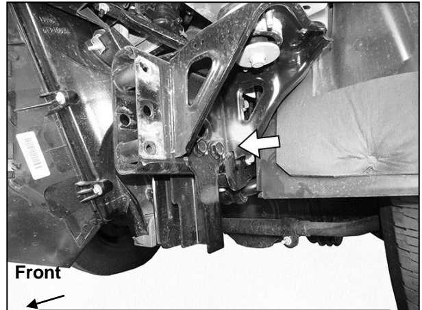
(Fig 2) Bumper removed. Also remove tow hooks and lower frame extensions as equipped (arrow)
