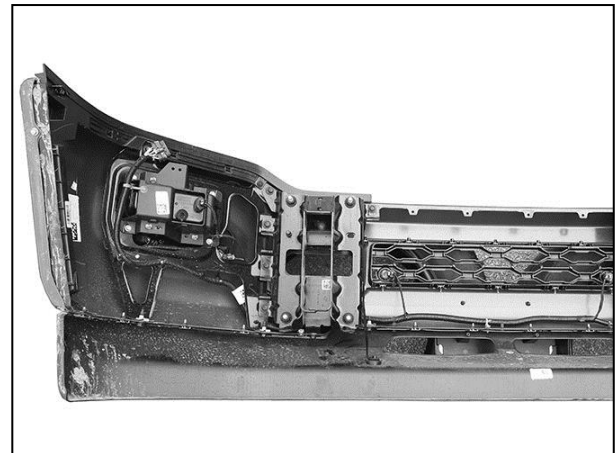
(Fig 8) Remove harness and parking sensors from factory bumper if equipped
