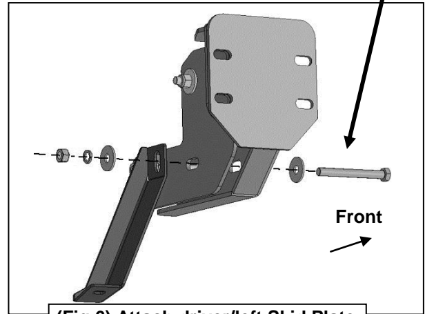
(Fig 6) Attach driver/left Skid Plate Bracket to Inner Frame Bracket
