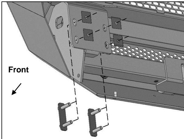
(Fig 15) Insert (2) Double Bolt Plates through back of mounting plate on Bumper
