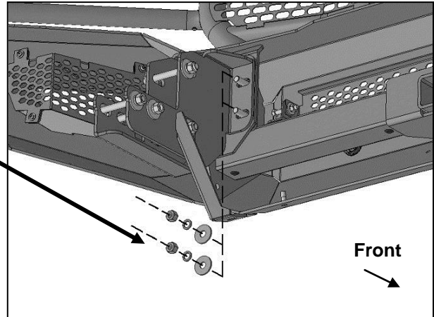
(Fig 18) Attach driver/left side of Bumper to Frame Brackets. Inner Bracket illustrated
