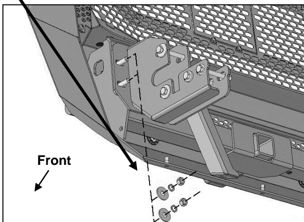
(Fig 17) Attach driver/left side of Bumper to Frame Brackets. Outer Bracket illustrated
