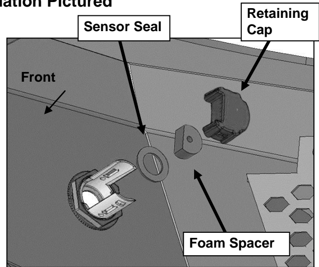
(Fig 10) Remove front seal from Sensor. Apply larger Foam Seal to sensor. Slide sensor into mount, insert Foam Spacer and Retaining Cap to lock sensor in mount
