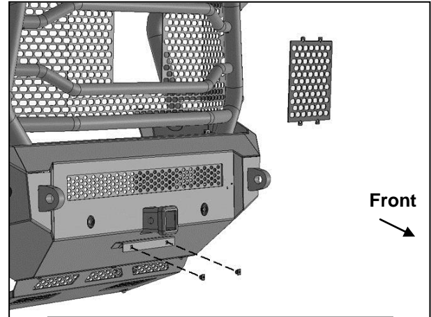
(Fig 22) Models with camera, remove panel from grille. Push Plastic Plugs into Bumper for license plate
