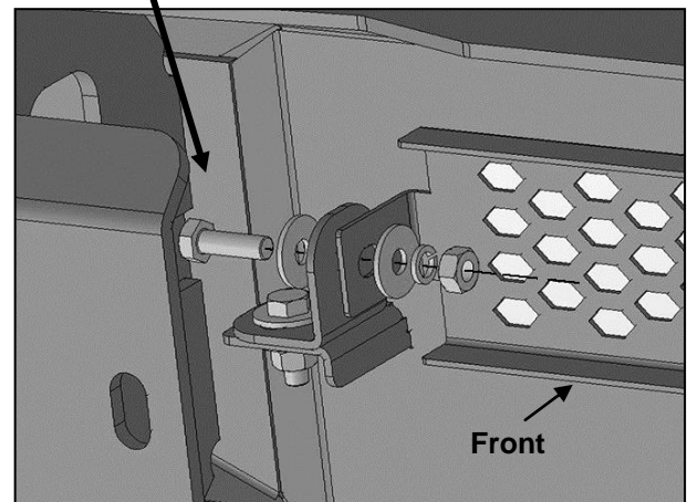
(Fig 12) Attach Mesh Fill Panel to "L" Brackets
