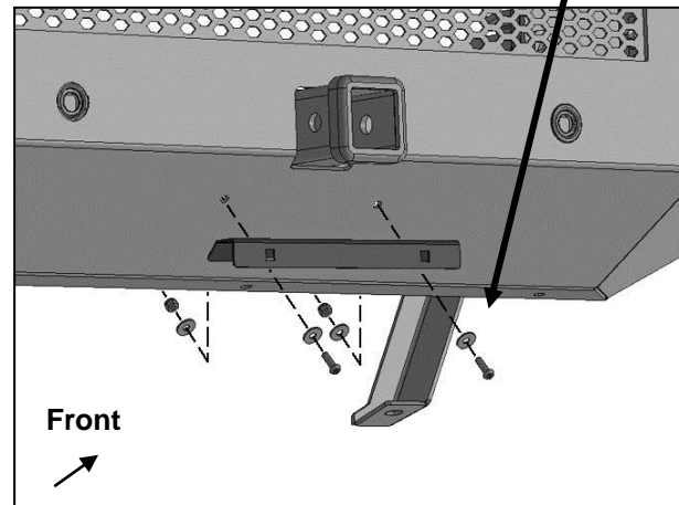
(Fig 20) Attach License Plate Bracket to Bumper before installing Skid Plate
