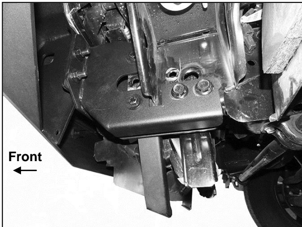
(Fig 19) Driver/left side of Bumper installed
