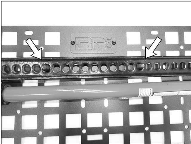
(Fig 7) Example of beam style recovery jack attachment to Carriage Bolts in Panel (arrows)
