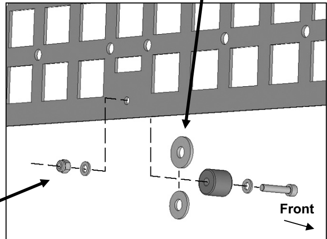
(Fig 4) Attach Rubber Bumper to front facing side of the Panel, between the Panel and the front of the bed. Use the 10mm Flat Washers to adjust the Bumper to touch the front of the bed.
