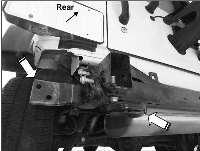
(Fig 3) Remove tow hook and outer bumper bracket from driver/left side of frame (arrows)
